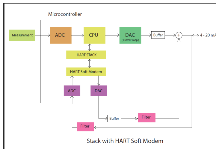
Example Block Diagram with Integrated Soft Modem
