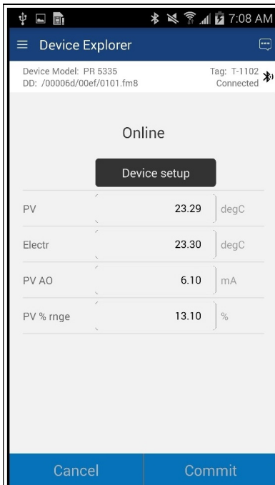
DevComDroid HART App + HM-USB-ISO HART Modem
