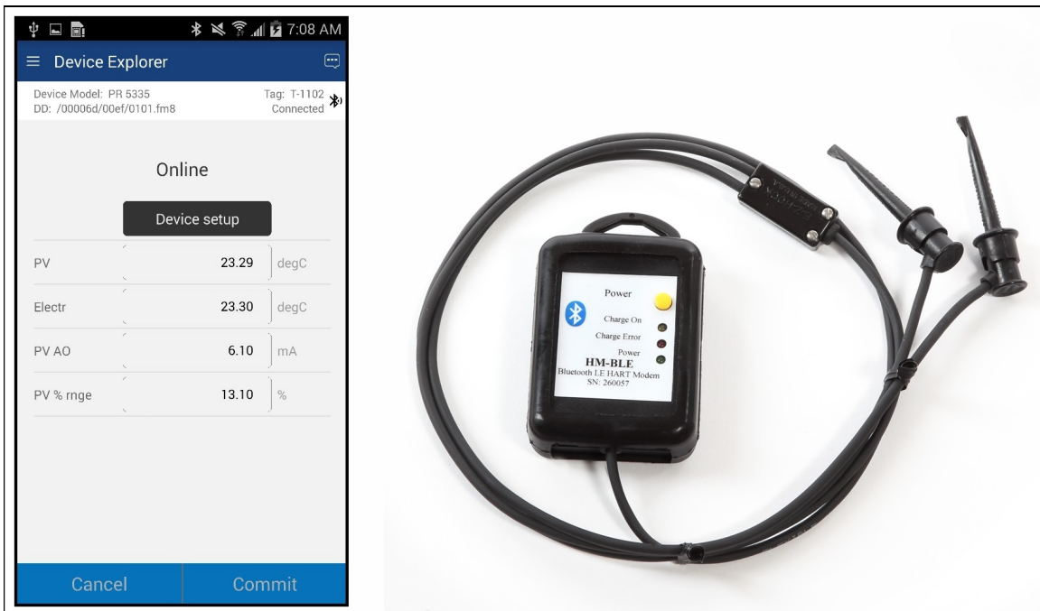
DevComDroid HART App + HM-BLE Bluetooth Low Energy HART Modem
